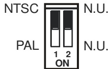
Figure 6: VP-501xl Dipswitches
