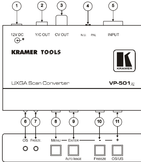
Figure 1: VP-501xl UXGA Scan Converter
