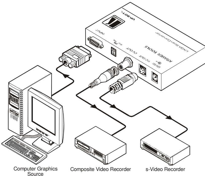
Figure 3: Connecting the VP-501xl
