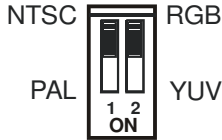
Figure 7: VP-502xl Dipswitches
