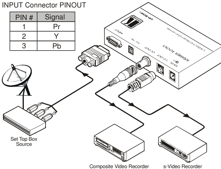
Figure A1: Connecting the VP-502xl
