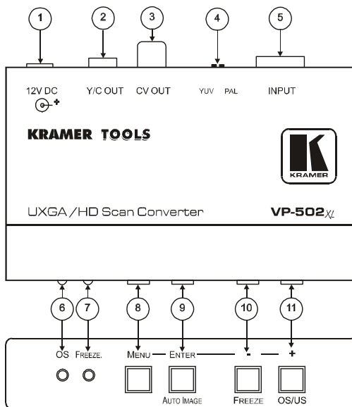
Figure 2: VP-502xl UXGA/HD Scan Converter
